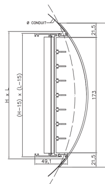
BCC H=200
