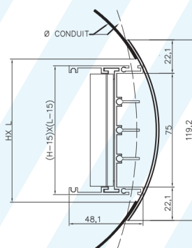
BCC H=100
